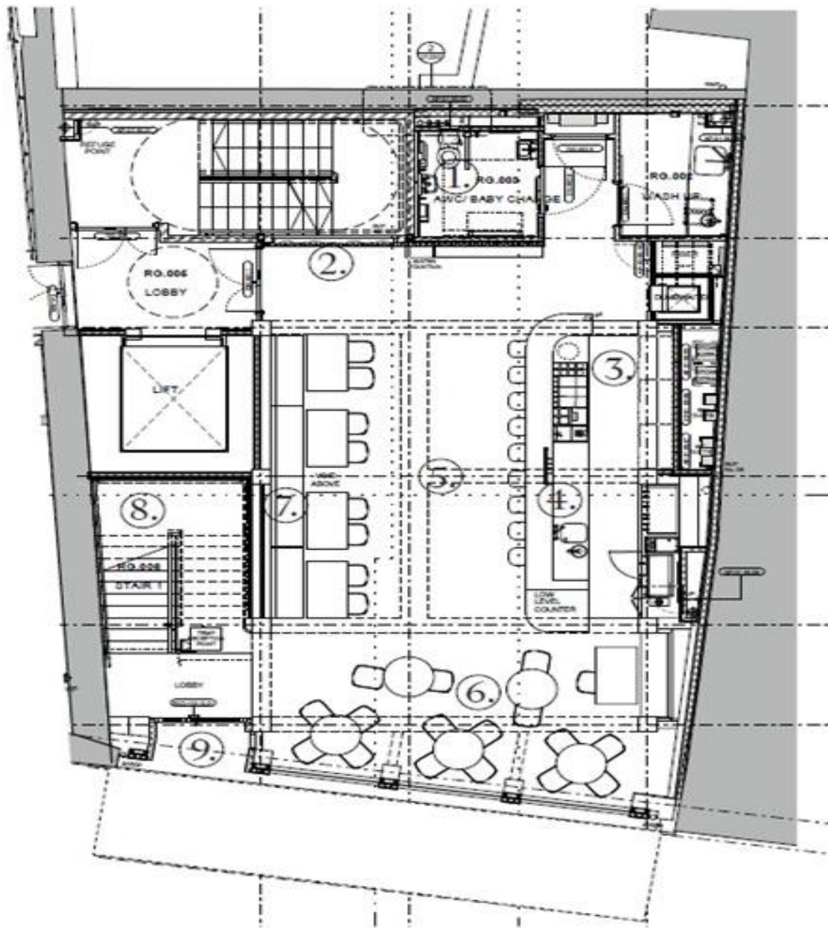
STAGE 4 - G+0 GROUND FLOOR PLAN
