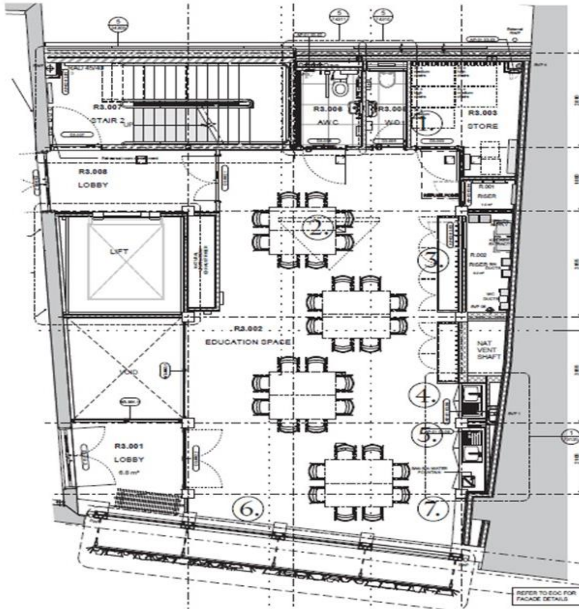
A STAGE 4 - G+3 THIRD FLOOR PLAN
